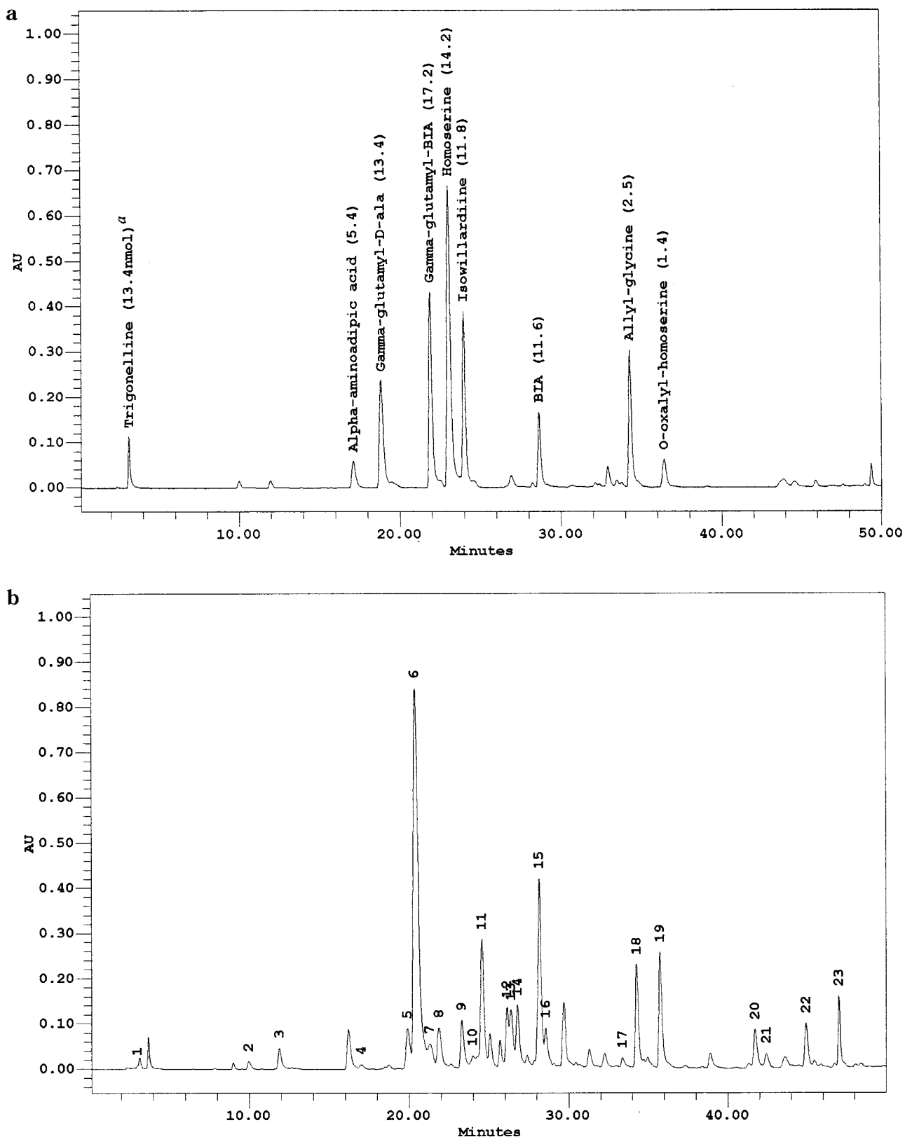
Figure 2. Chromatograms of nonprotein amino acid standards (a) and total amino acids in lentil seedlings (b) by HPLC. Peaks: 1, trigonelline; 2, Asp; 3, Glu; 4, \alpha -aminoadipic acid; 5, Ser; 6, Asn; 7, Gly; 8, \gamma -glutamyl-BIA; 9, Hse; 10, isowillardiine; 11, His; 12, Arg; 13, Thr; 14, Ala; 15, Pro; 16, BIA; 17, Tyr; 18, allylglycine (internal standard); 19, Val; 20, Ile; 21, Leu; 22, Phe; 23, Lys. Peaks without numbers are unidentified compounds. a The nanomoles injected are shown in parentheses.
